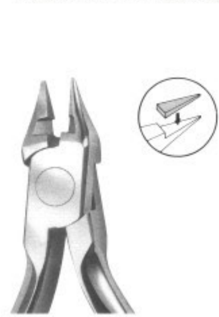
2661 Bird Beak Plier With Cutter Maximum Bending & Cutting Capacity: Wires up to .032"
