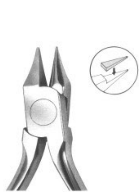
2662 Bird Beak Plier Maximum Bending Capacity: Wires up to .032"
