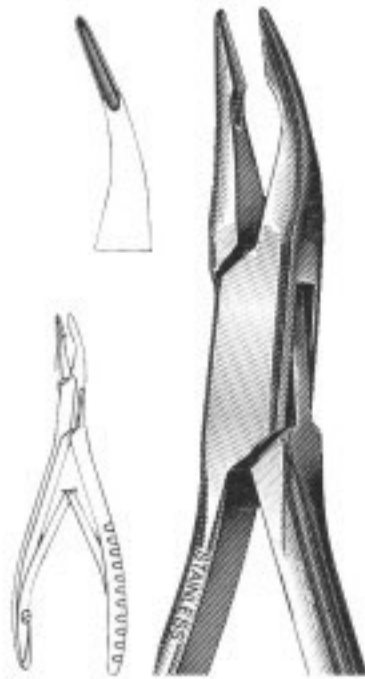
2758 MICRO-FRIEDMAN 5 1/2", 15° Curved Jaws
